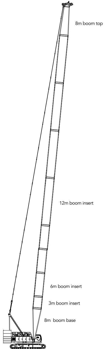
H Configuration 16m-85m
