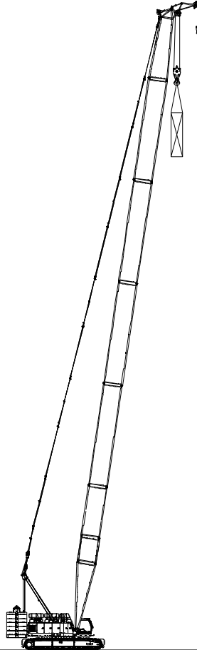
HCm Configuration (double hooks, load on main hook)
