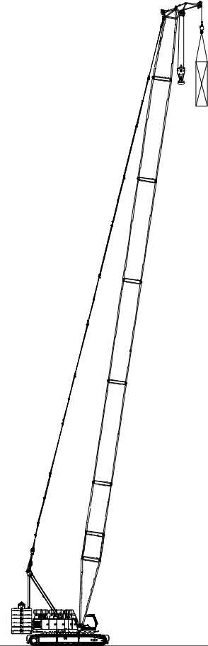
HCa Configuration (double hooks, load on aux. hook)
