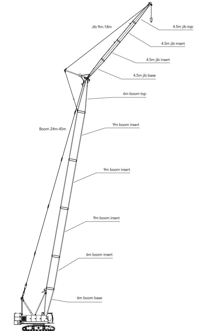
FJ Configuration (Longest boom+ jib: 45m+18m)
